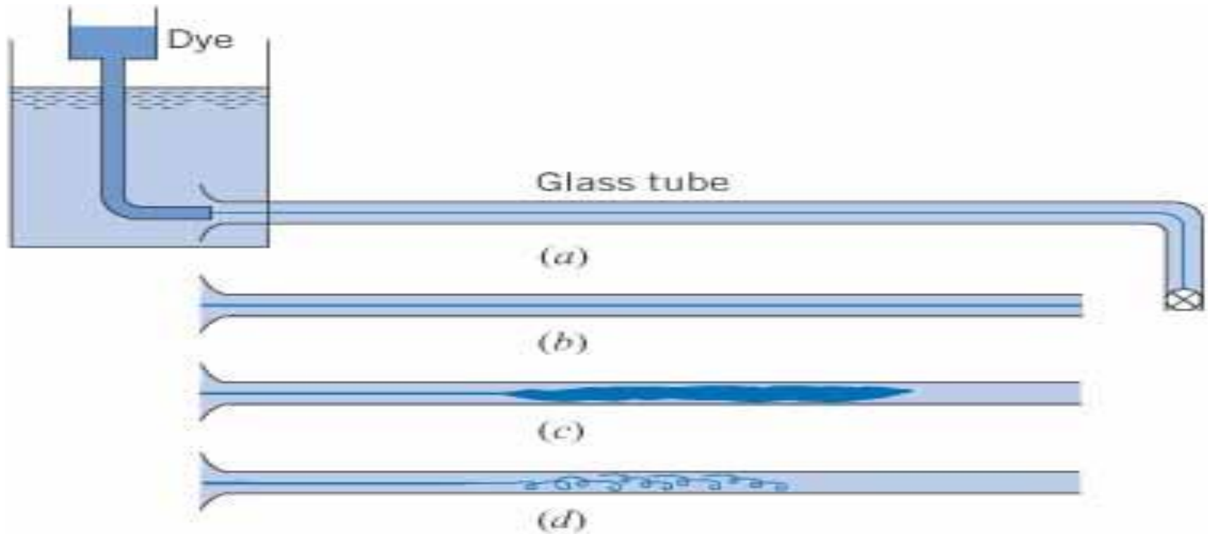
Figure 10.1 Reynolds' experiment.
