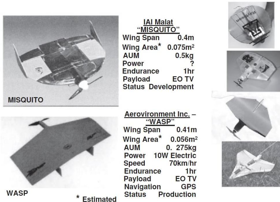
Figure 3.20: Micro air vehicle systems (Reproduced by permission of AeroVironment Inc)
