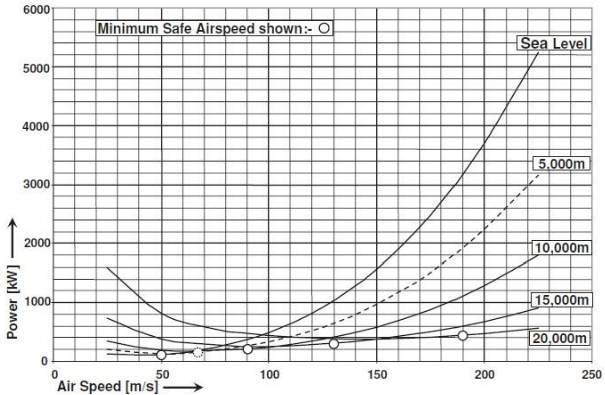
Figure 3.7: HALE UAV: power required to maintain height. Variation with airspeed and altitude – 81.8 kN AUW, ISA conditions
