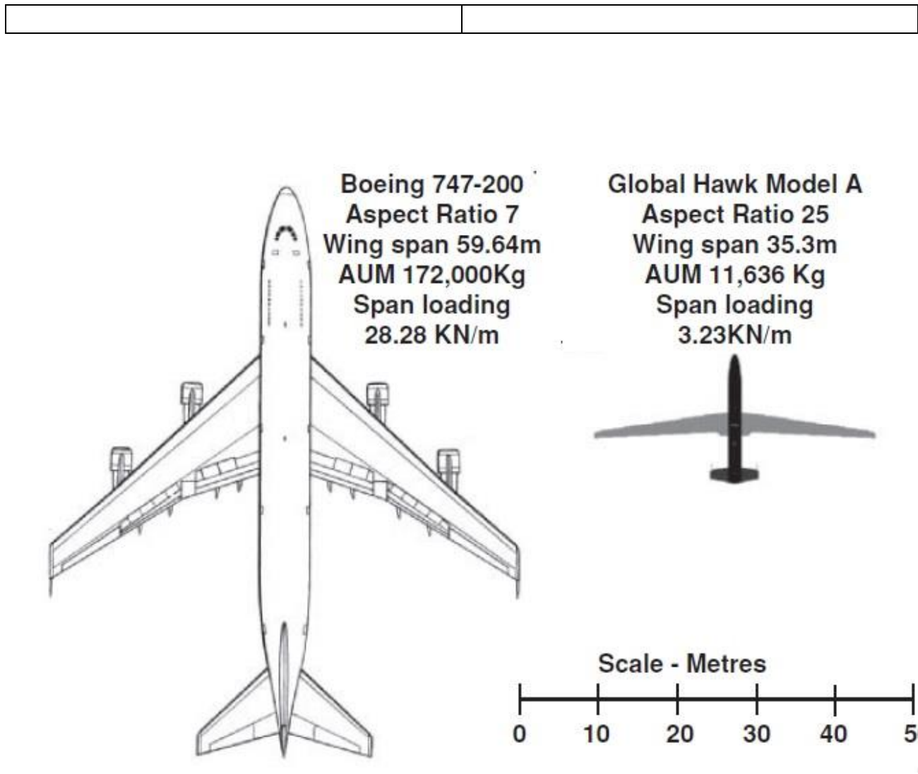
Figure 3.2: Comparison of wing aspect ratios
