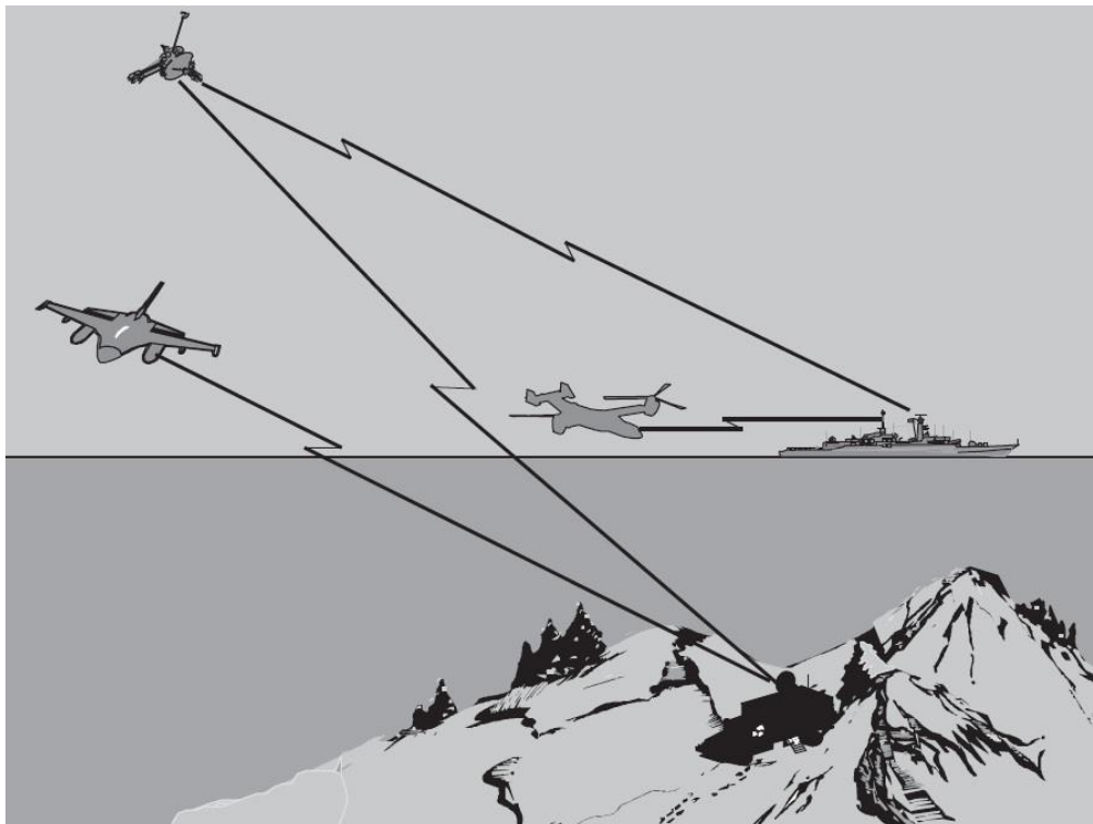
Figure 4.4: Interoperable systems
