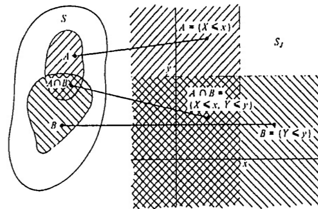
Comparison of sample space s with s_j
