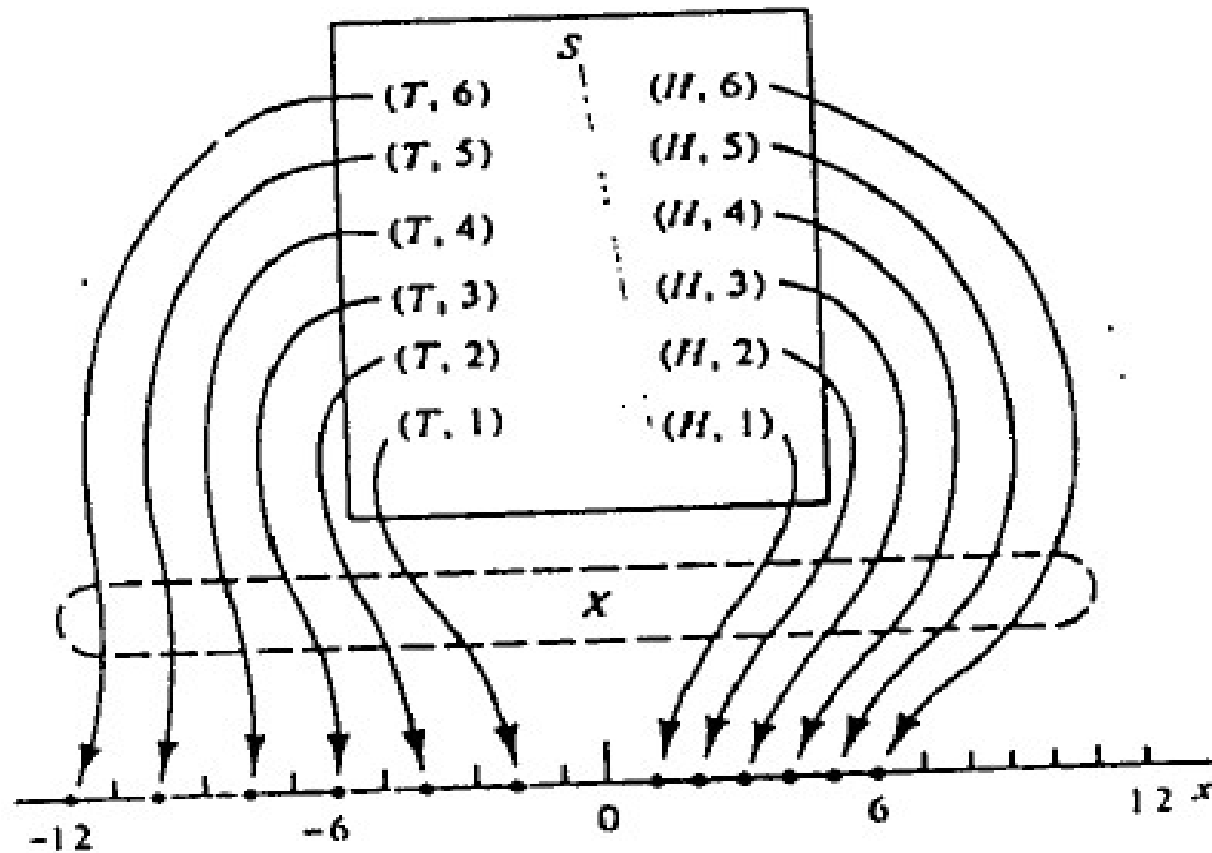
Mapping of sample space to a real line
