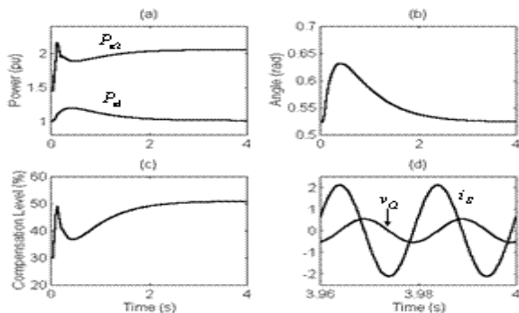
Fig. 10.19 System response with regulating power flow controller
