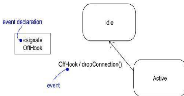
Fig: Event
