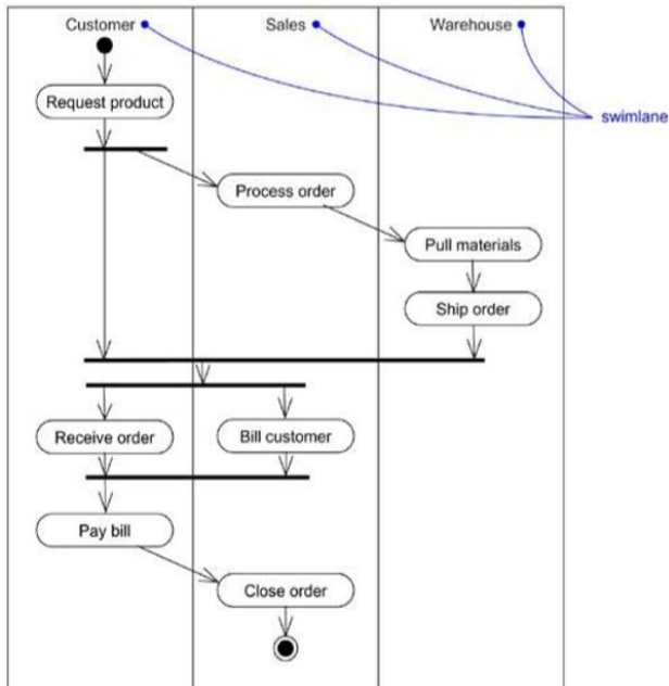
Fig: Swimlanes
