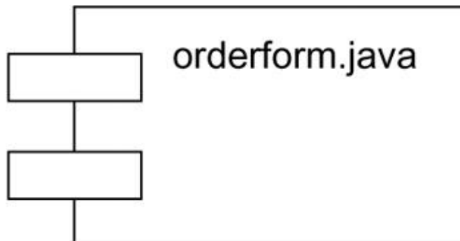
Figure :Components
