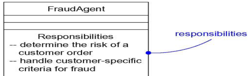
Fig: Responsibilities
