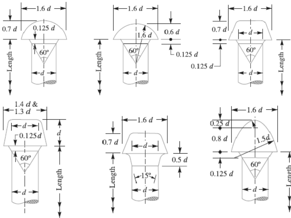
Fig. Rivet heads for general purposes (from 12 mm to 48 mm diameter)
