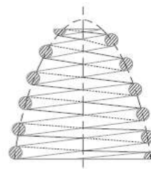
(b) Volute spring.
