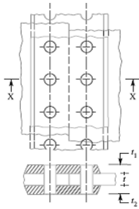
Fig. Single riveted double strap butt joint.
