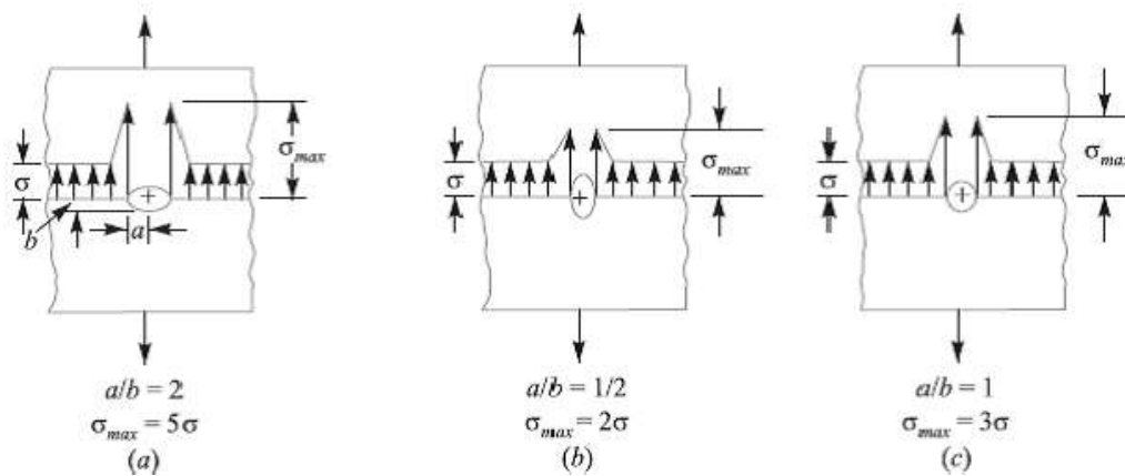
Fig.1. Stress concentration due to holes.
