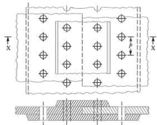
Fig. Double riveted double strap (unequal) butt joint with zig-zag riveting.
