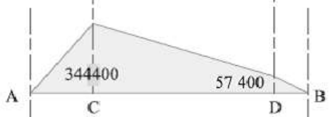
(e) Vertical B.M. diagram.
