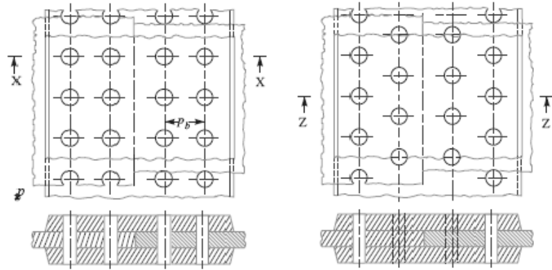
Fig. Double riveted double strap (equal) butt joints.
