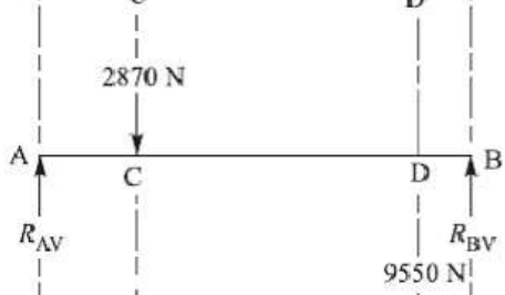
(c) Vertical load diagram.
