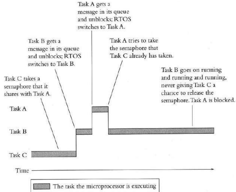
Figure 6.17 Priority Inversion
