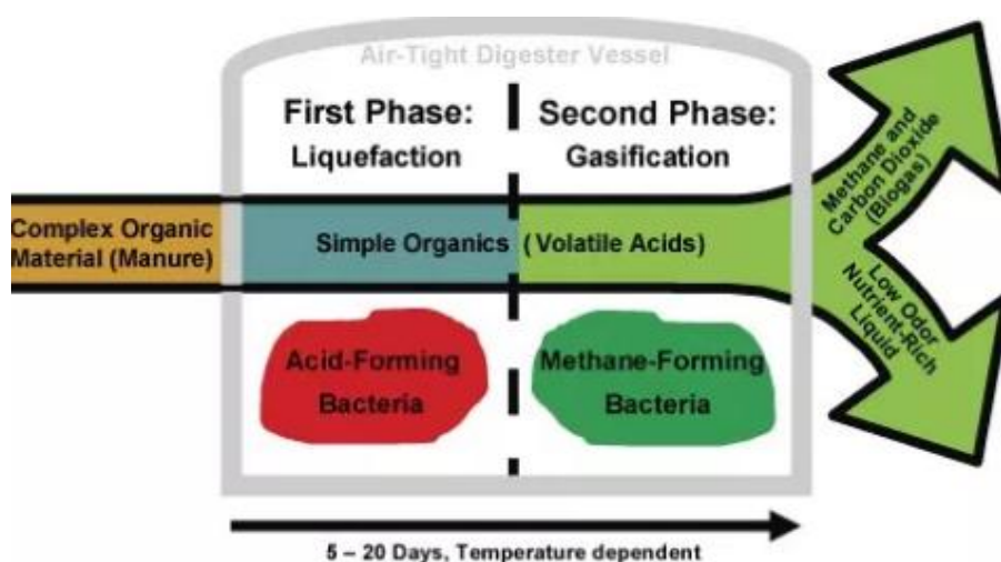
Fig.3.1. Working of anaerobic digestion
