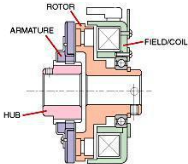
Fig: Electromagnetic Clutch
