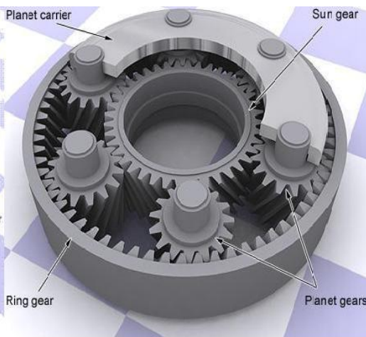
Figure 10 Planetary Gear Set.
