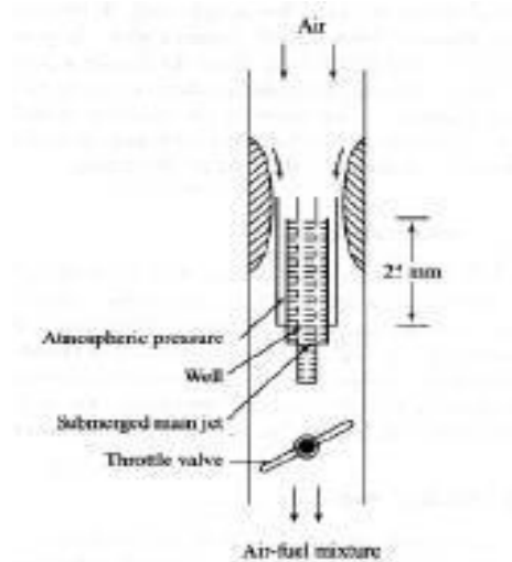
Figure: 6 Emulsion Tube
