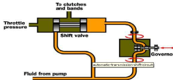
Fig: Hydraulic System
