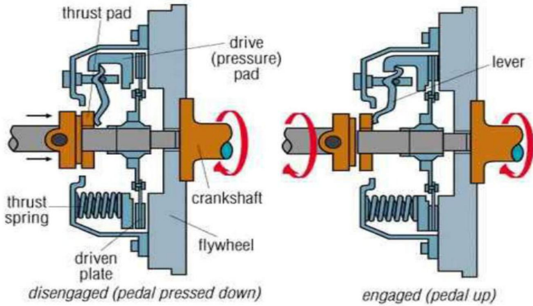
Fig: Clutch in Engaged & Disengaged Position
