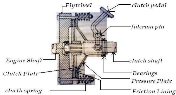
Fig: Single Plate Clutch
