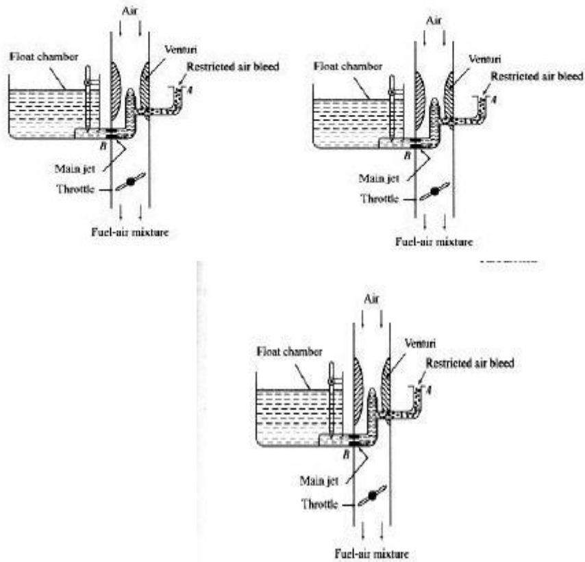
Figure: 4 Air bleed principle in a typical carburetor
