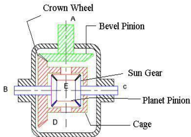
Fig: Differential gear Assembly
