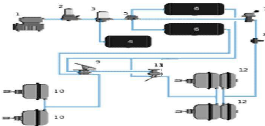
Highly simplified air brake diagram on a commercial road vehicle (does not show all air
