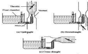
Figure: 8 Types of Carburetors
