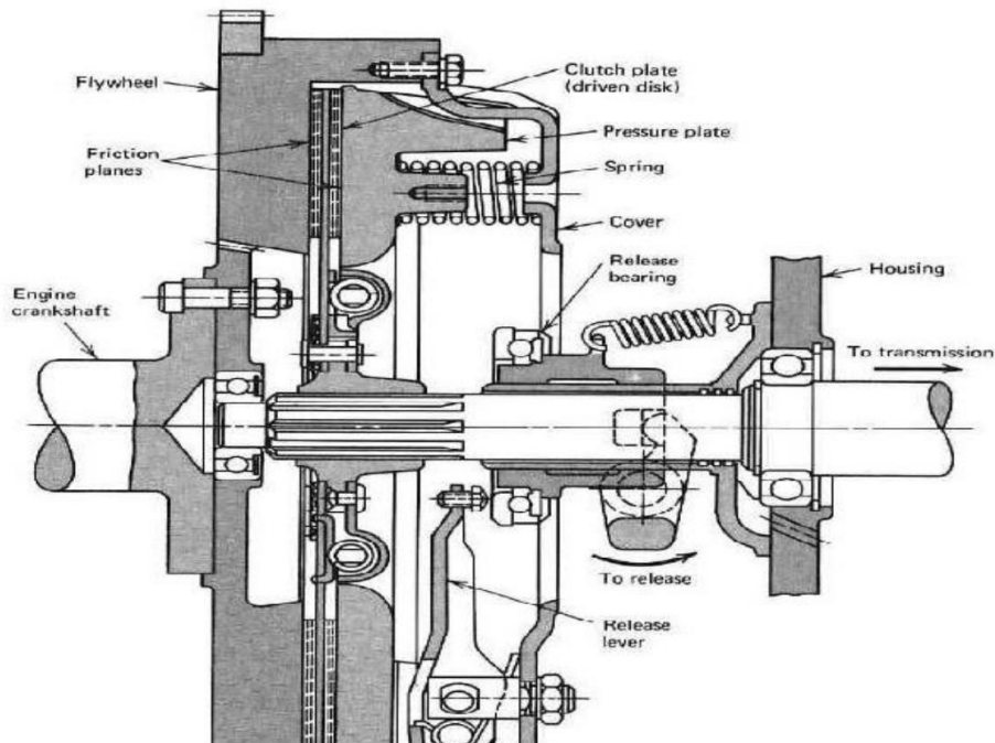
Fig: Clutch in Engaged & Disengaged Position
