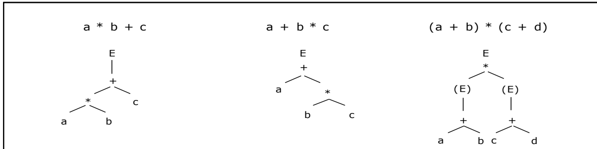
Syntax Trees
