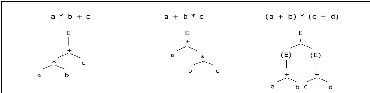
Syntax Trees
