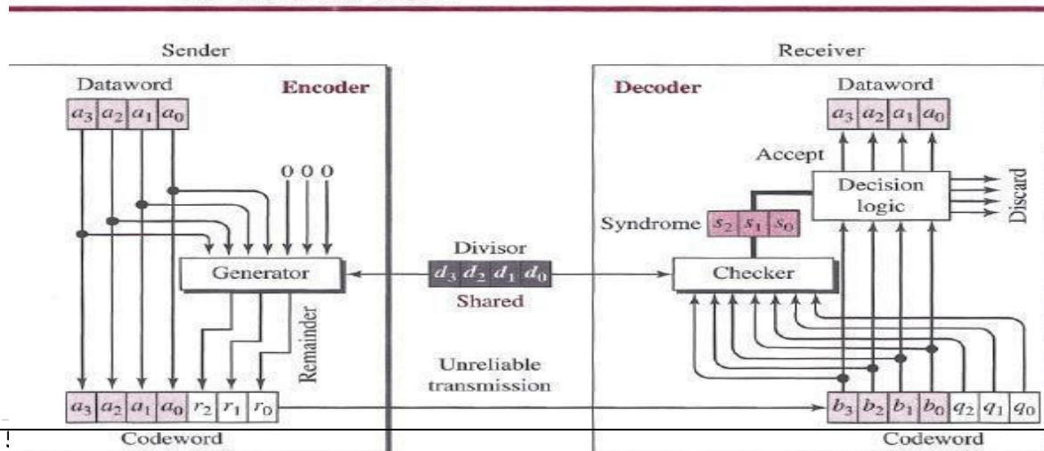
CRC encoder and decoder
