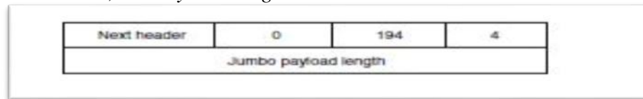
Figure: The hop-by-hop extension header for large data grams (jumbo grams)
