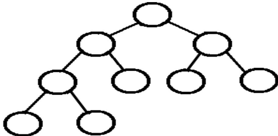
complete tree
