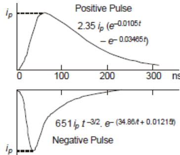
Fig. 3.4 Single positive and negative pulses
