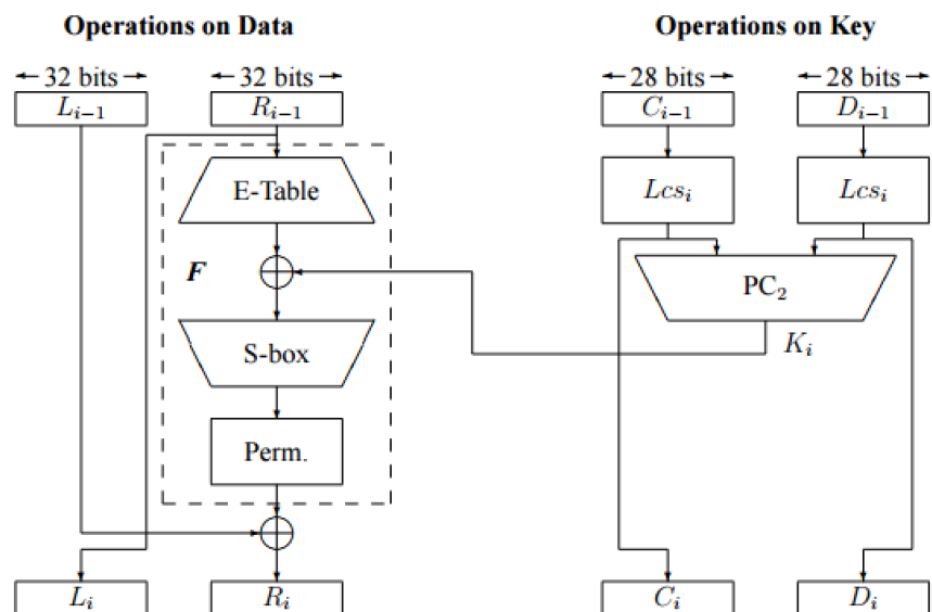
Figure : Details of a single DES round.
