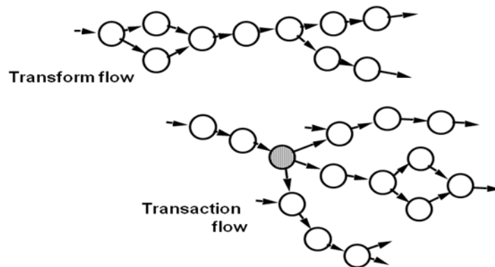
Flow Characteristics
