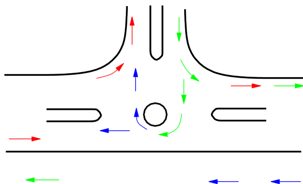
Figure 27:2: Channelization of traffic through a three-legged intersection
