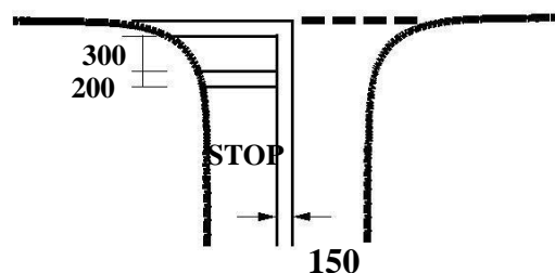
Figure 10: Stop line marking near an intersection
