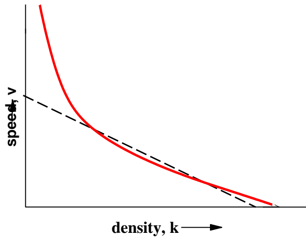
Figure 12: Greenberg's logarithmic model
