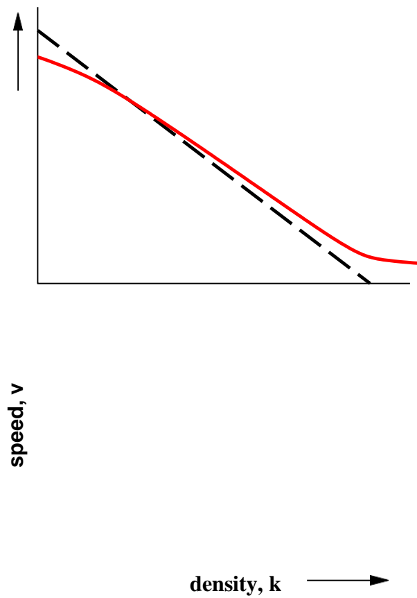
Figure 13: Underwood's exponential model
