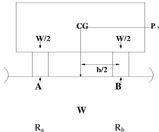
Figure 2: Effect of horizontal curve
