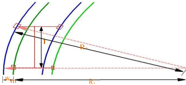
Figure 15:1: Extra-widening at a horizontal curve
