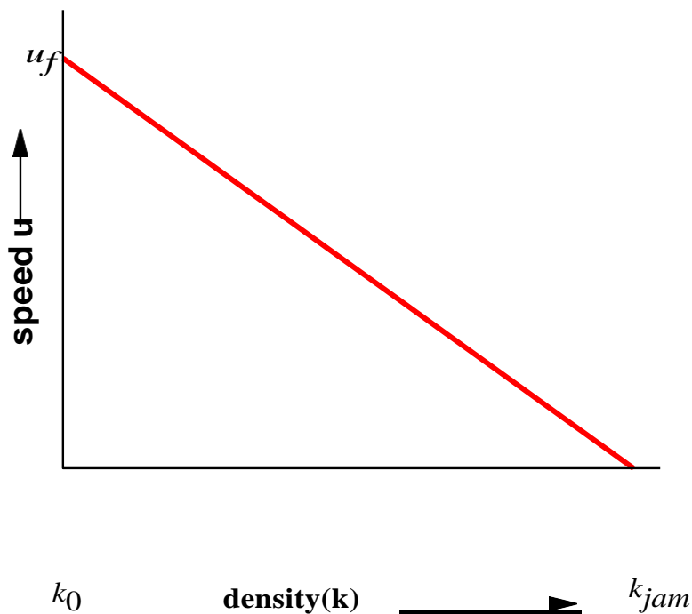
Figure 12: Relation between speed and density
