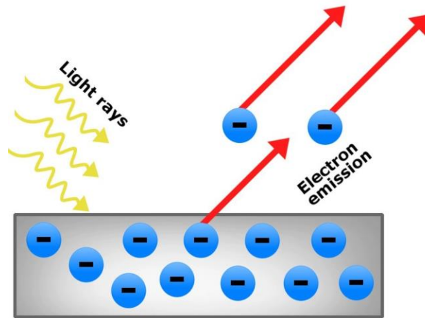
Figure 3 Photoelectric effect
