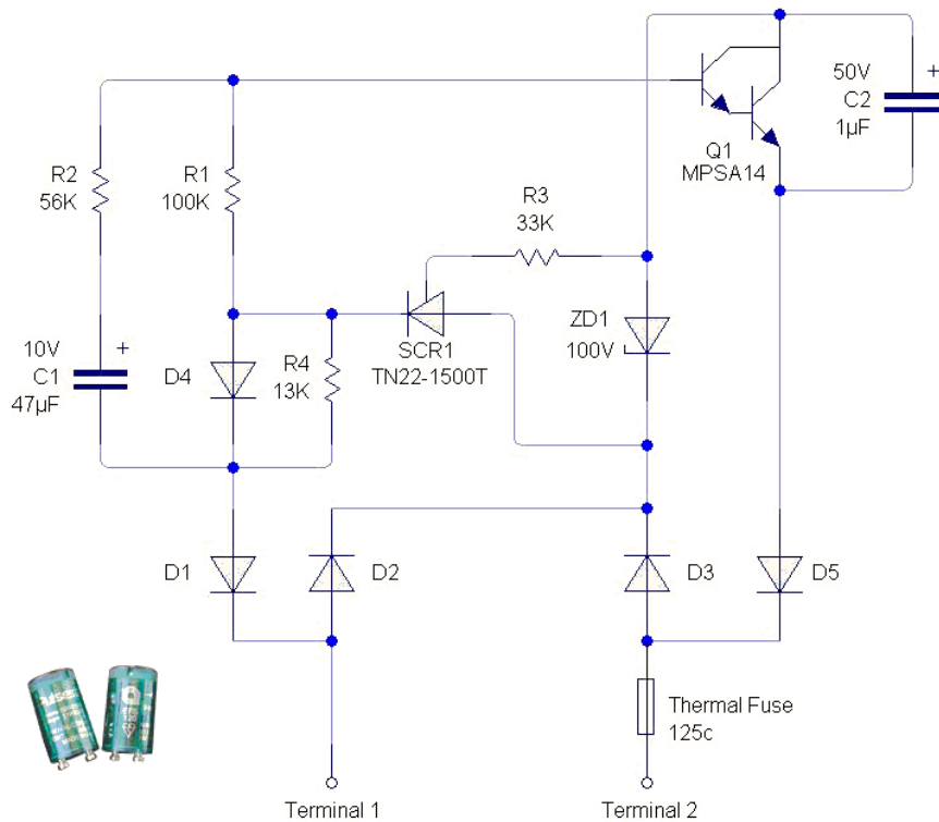
Arlen EFS-120 "Pulsestarter"
