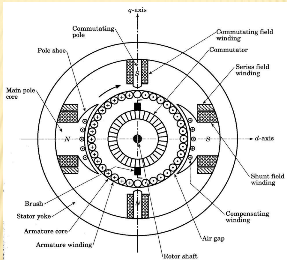
General arrangement of a dc machine
