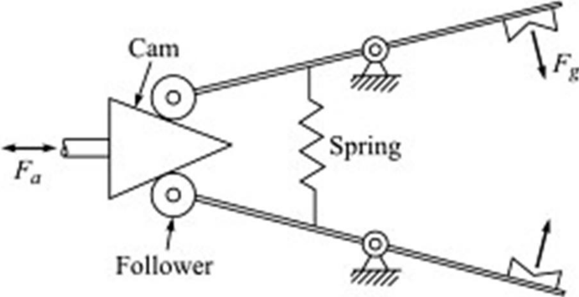
Cam-actuated gripper.
