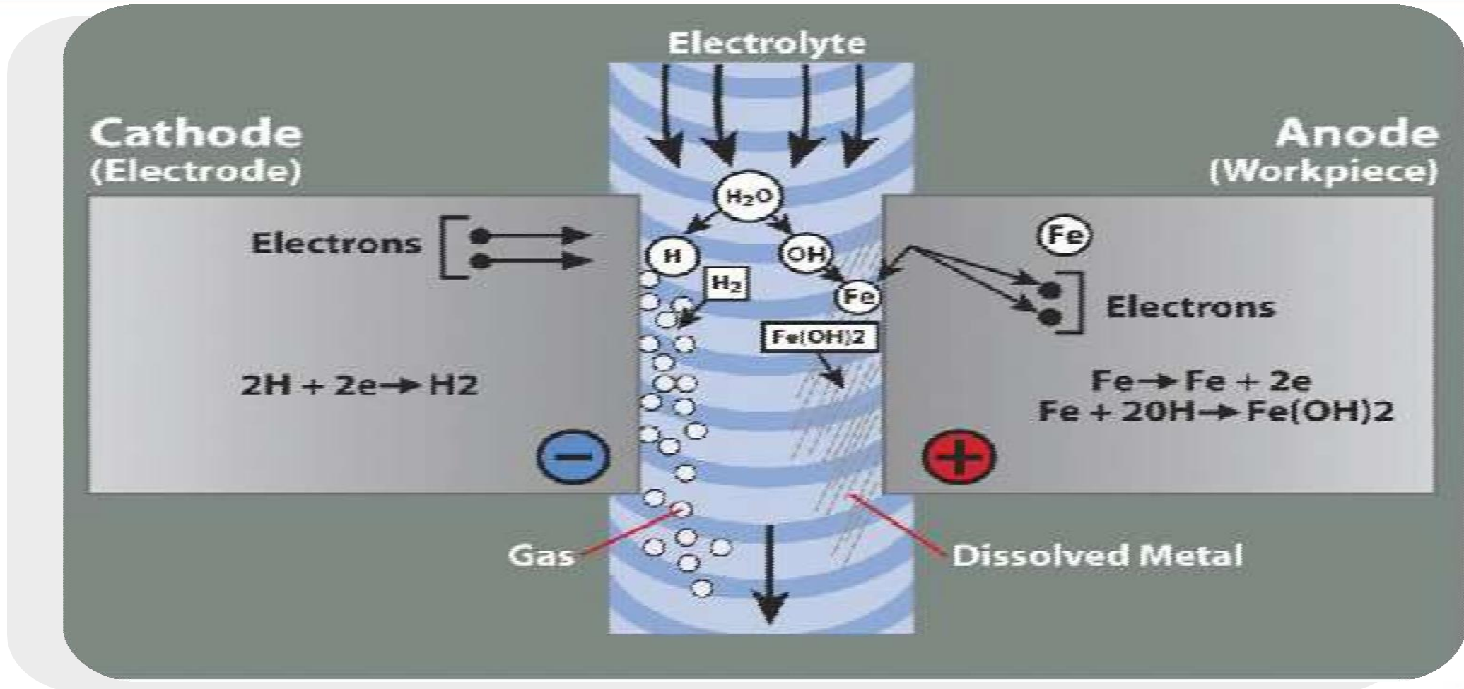
Fig : ELECTROCHEMICAL HONING
