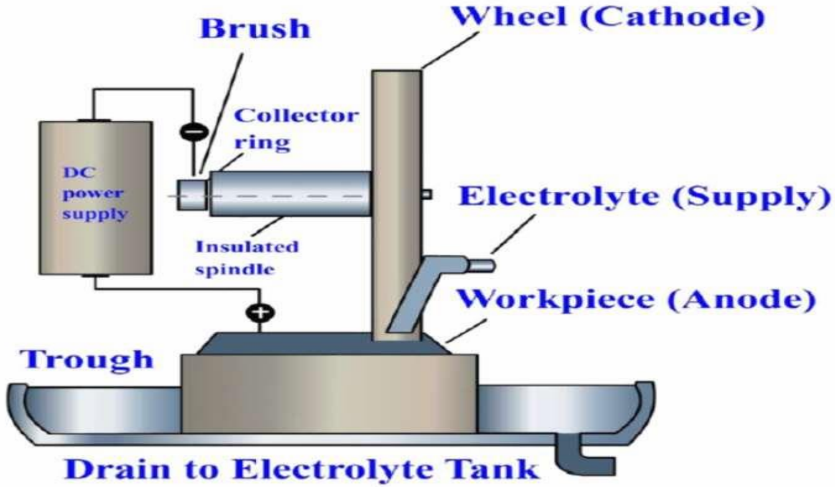
Fig: SCHEMATIC VIEW OF ECG
