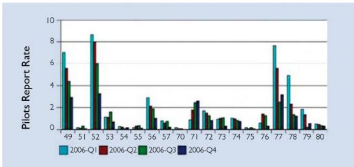
FIGURES 2 AND 3. PILOT REPORTS RATE FOR ATA CHAPTERS 21–38 AND 49–80. Analysis of Reliability Monitoring by Manufacturer of One Aircraft Type
