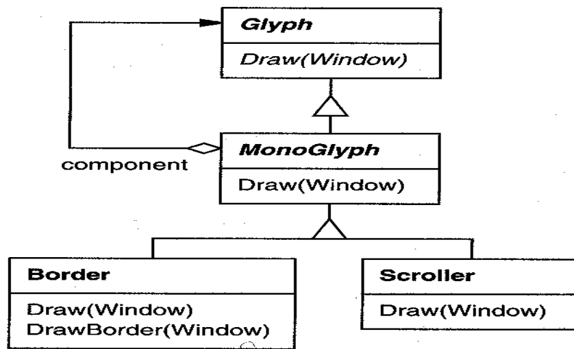
Figure 2.7: MonoGlyph class relationships
