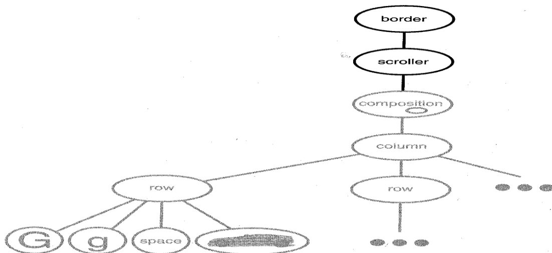
Figure 2.8: Embellished object structure
