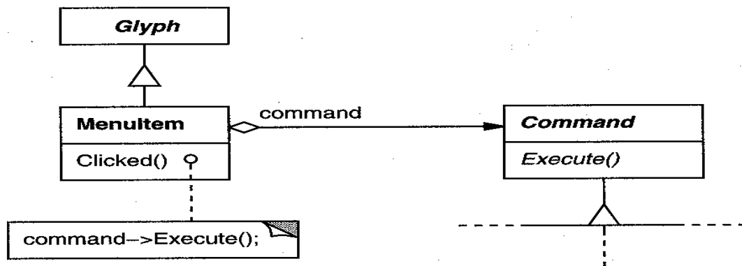
Figure 2.12: MenuItem-Command relationship
