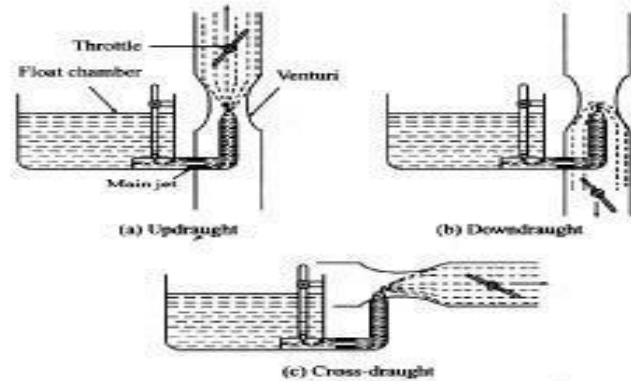
Figure: 8 Types of Carburetors
