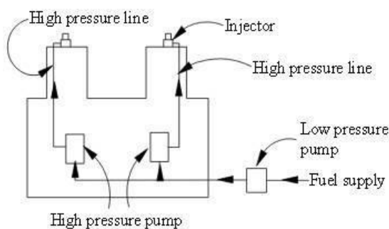
Separate pumps
