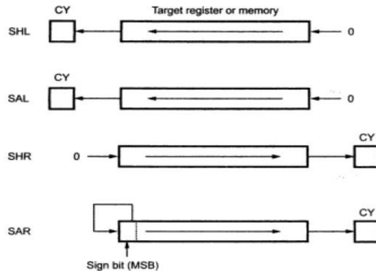
Fig.1 Shift operations
