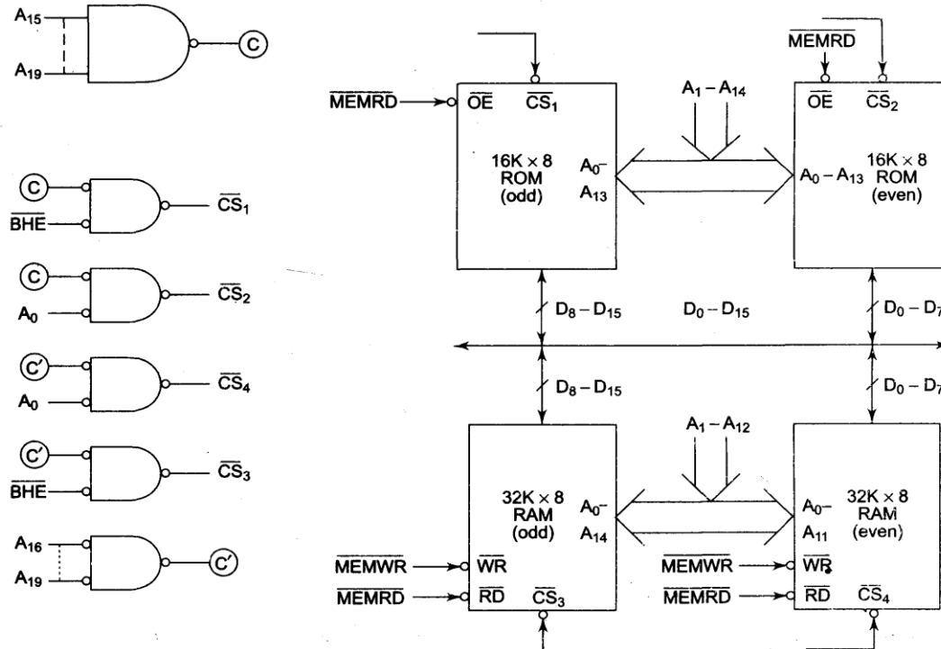
Fig. 5.2 Interfacing Problem 5.2
