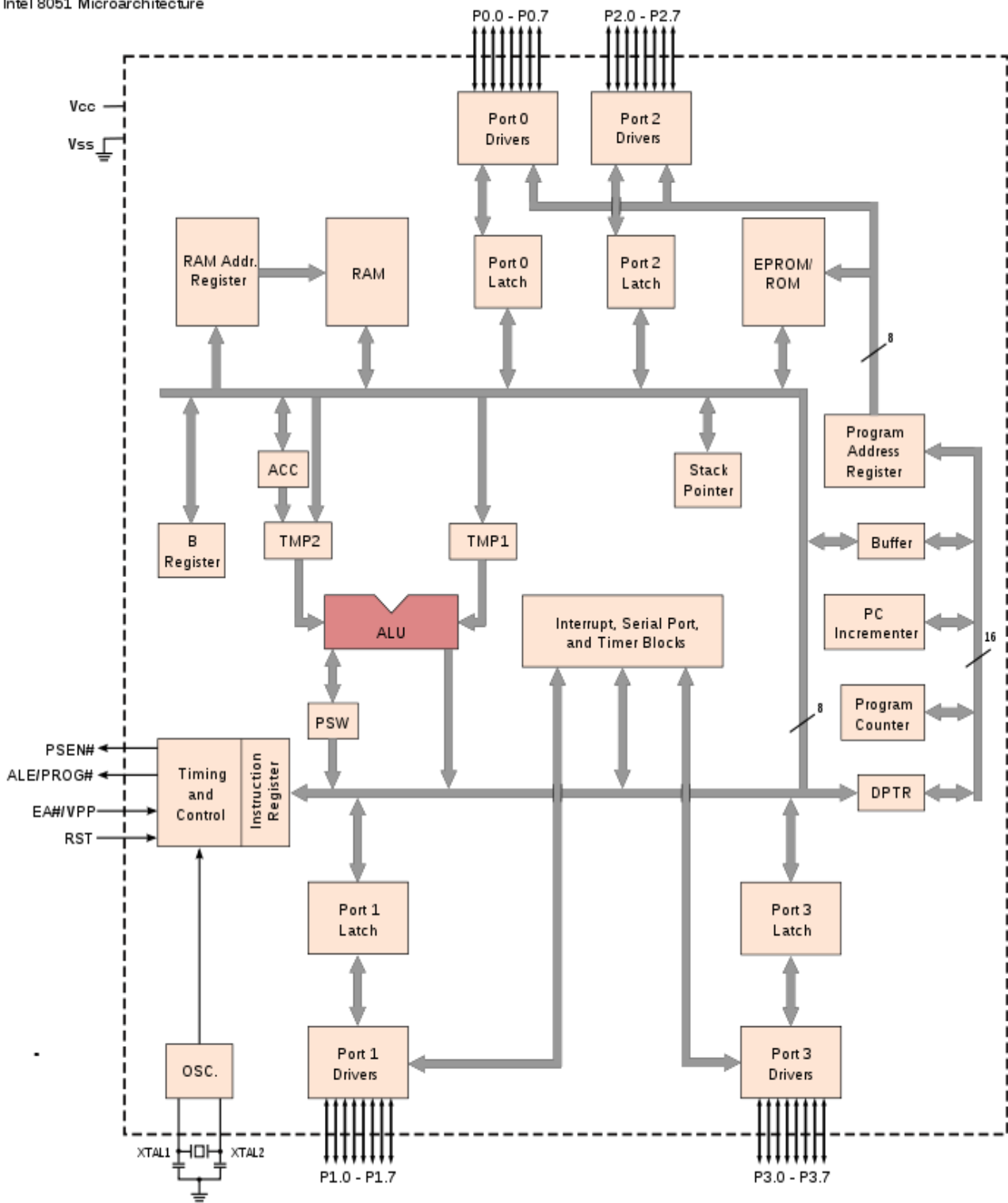
Intel 8051 Microarchitecture
