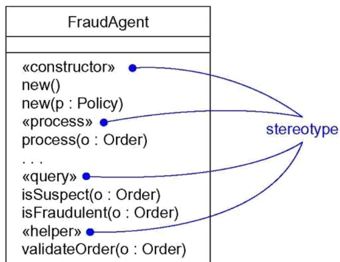
Figure Stereotypes for Class Features
