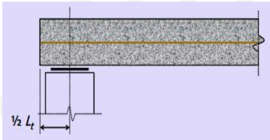
Figure 7-1.5 End of a simply supported member
