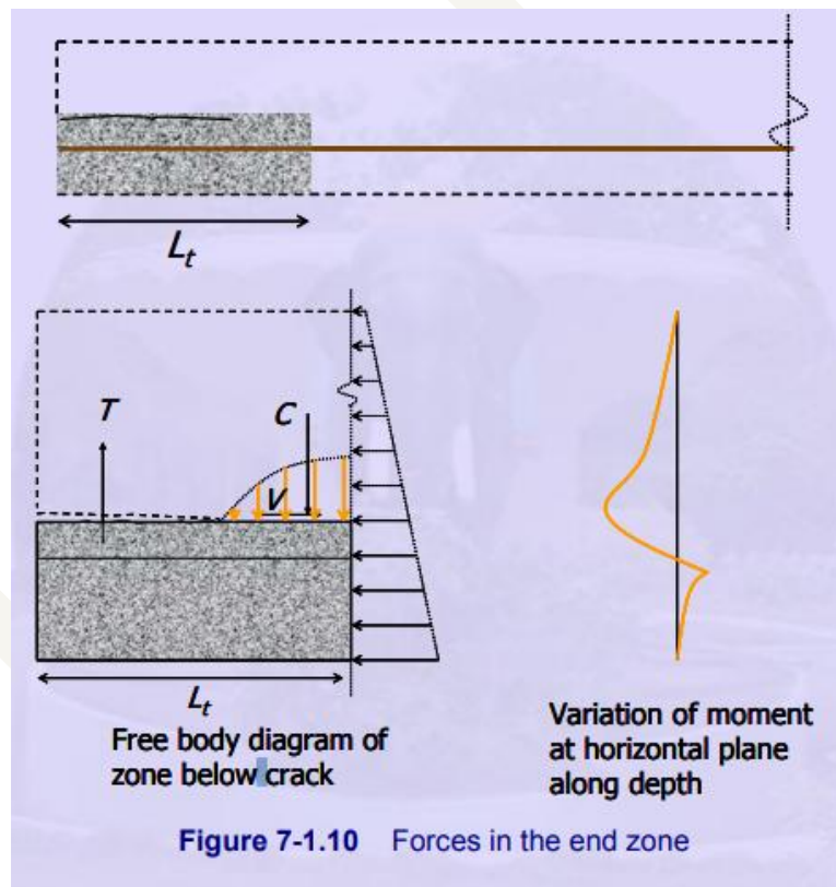
Figure 7-1.10 Forces in the end zone
