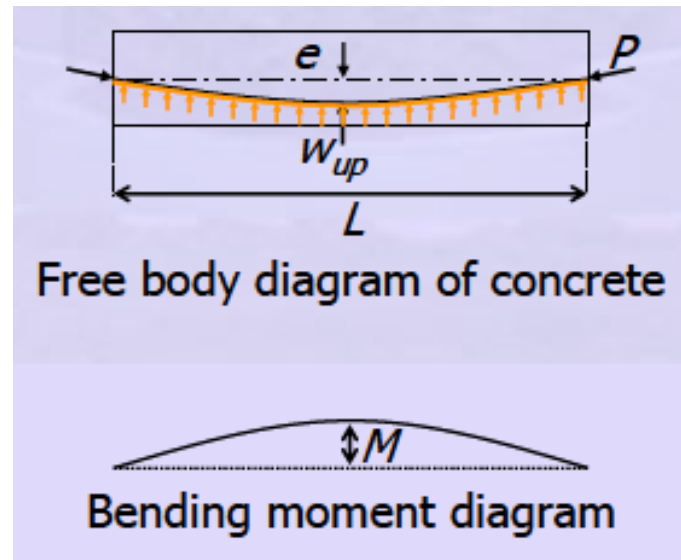
Simply supported beam with parabolic tendon
