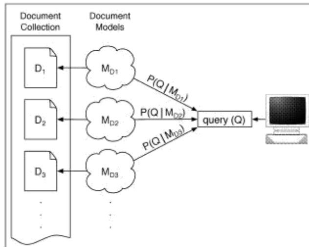
Fig: Documents collection
