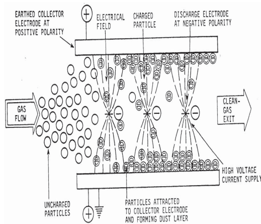
Figure 66: Electrostatic Precipitator
