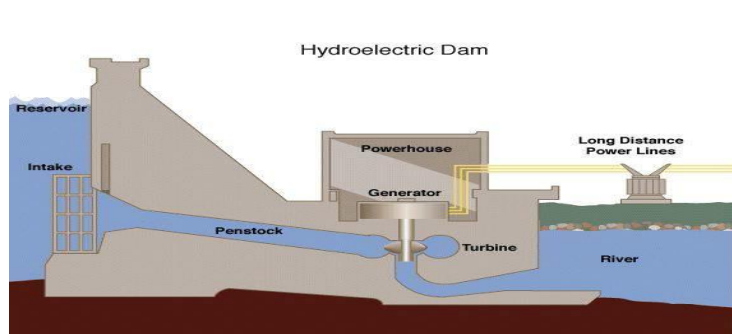
Figure: Schematic of a Hydropower Plant
