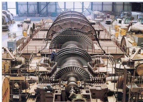
Figure: Steam Turbines
