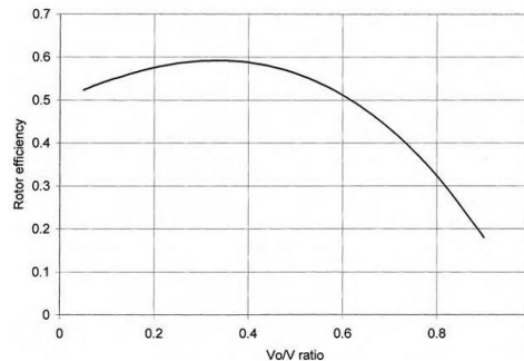
Figure: Rotor efficiency vs. Vo/V ratio has a single maximum.
