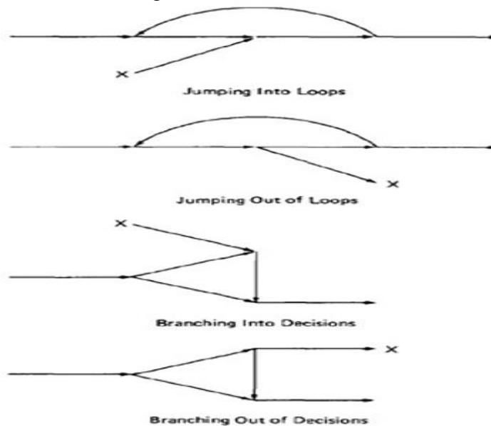
Figure 5.8: Un-structured sub-graphs.
